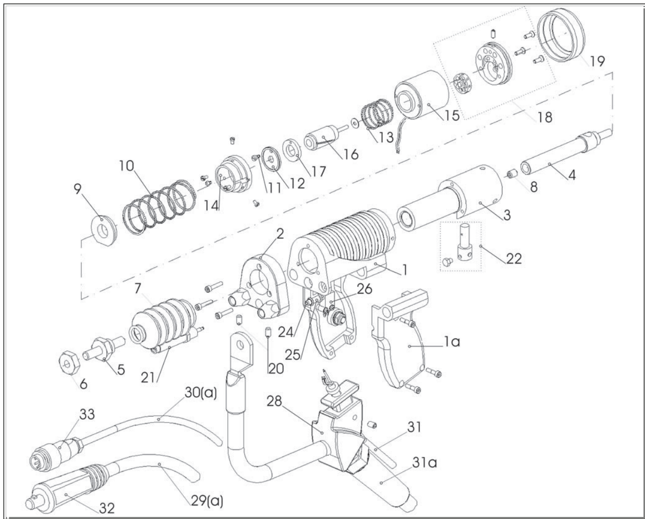
Figure 32: Exploded view of gun K 24
