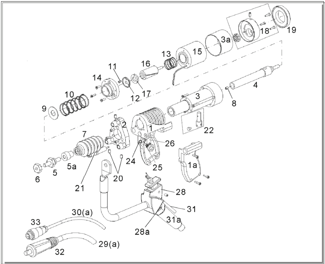
Figure 33: Exploded view of gun K 26 (from no. 400130)
